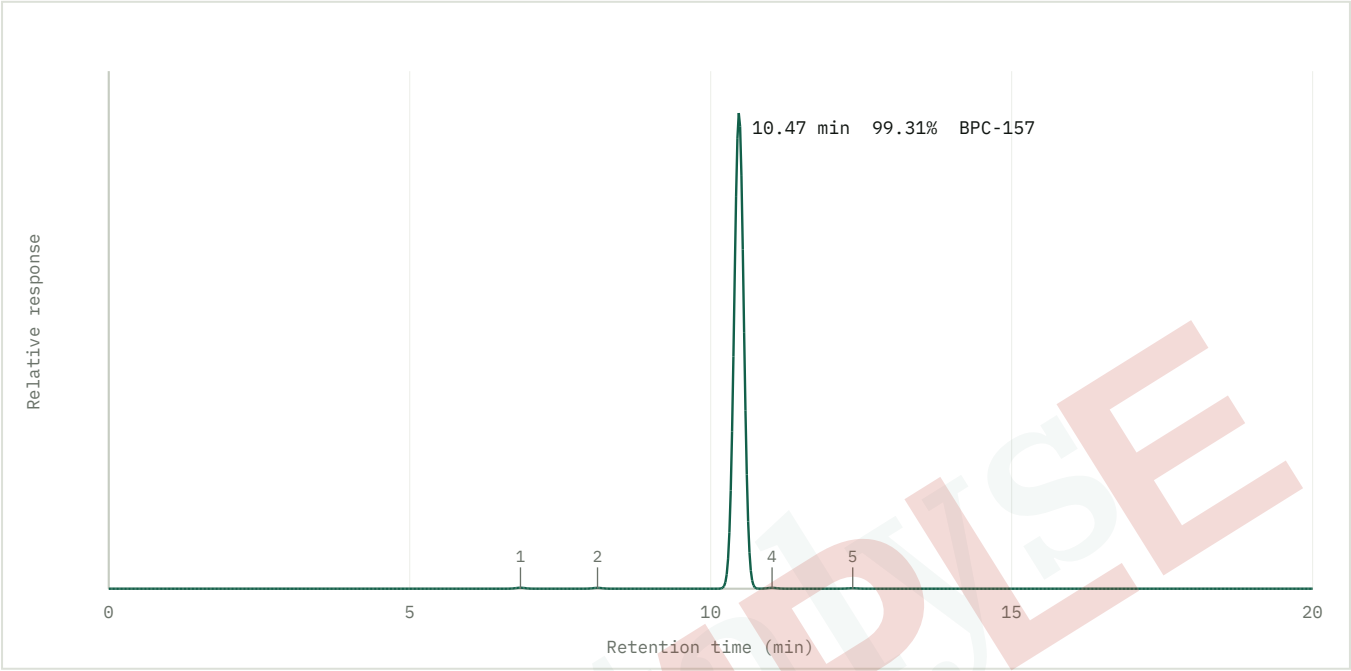
Figure 1 Chromatogram
